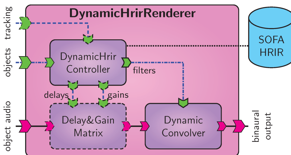
Fig. 4: Dynamic binaural synthesis rendering component. Optional parts are dashed.
